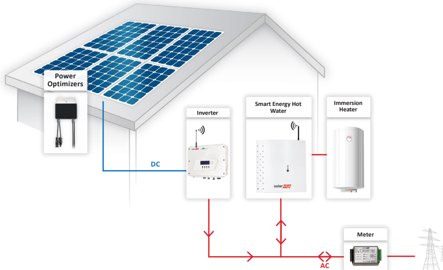
SolarEdge System with Smart Energy Hot Water
